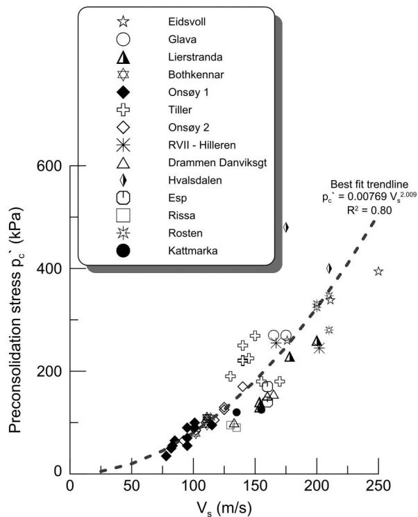
Fig. 17. Preconsolidation stress ( p'_c ) versus V_s
